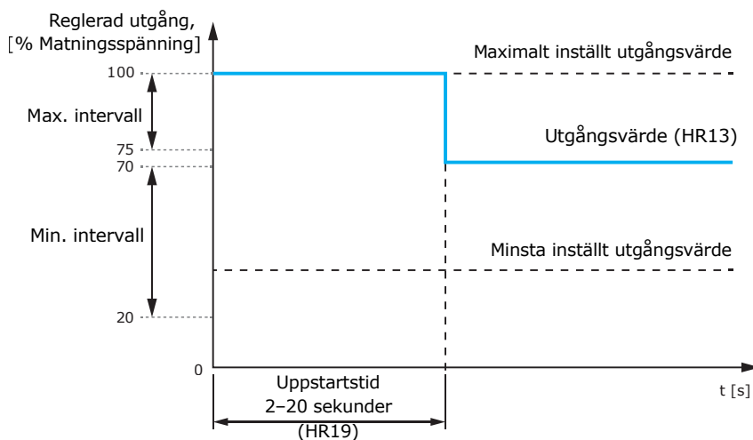
Fig. 5 Driftdiagram - Kickstart
