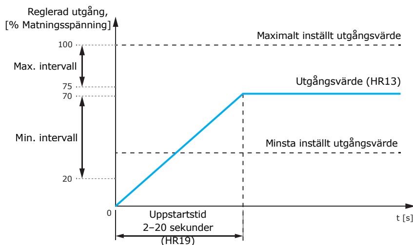
Fig. 5 Driftdiagram - Kickstart
