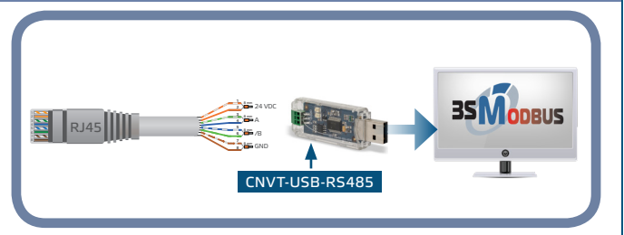
Fig. 5 RJ45-connectoren
