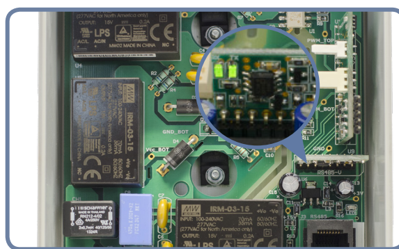
Fig.8 Communicatie LED indicatie
