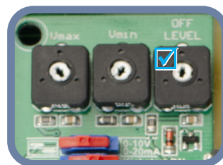
Fig. 7 Trimmer off-level
