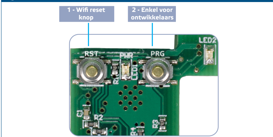
Fig. 5 - Wifi reset microschakelaar
