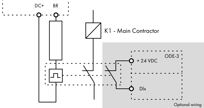
Thermal Overload / Brake Resistor with internal Over Temperature switch
