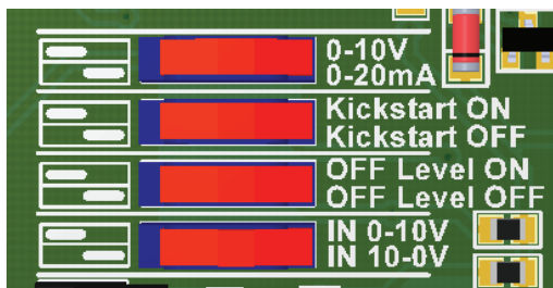
Fig. 4 DIP switch settings
