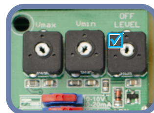
Fig. 7 Off level trimmer
