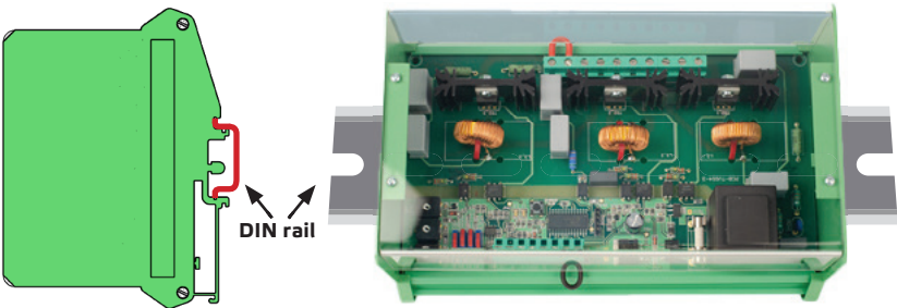
Fig. 2 Mounting position
