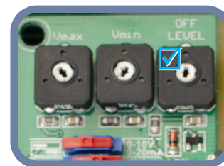
Fig. 7 Off level trimmer
