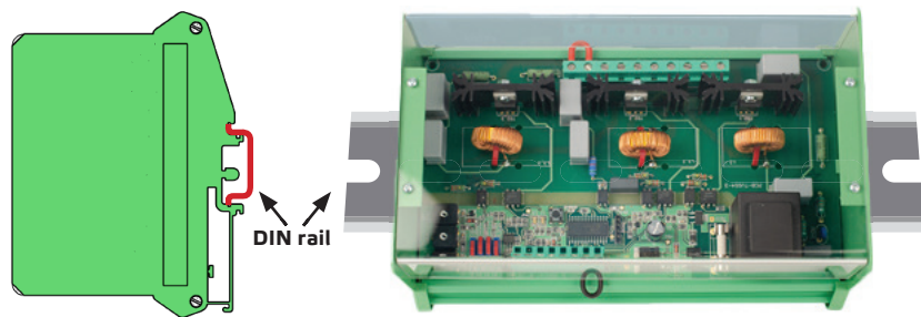
Fig. 2 Mounting position
