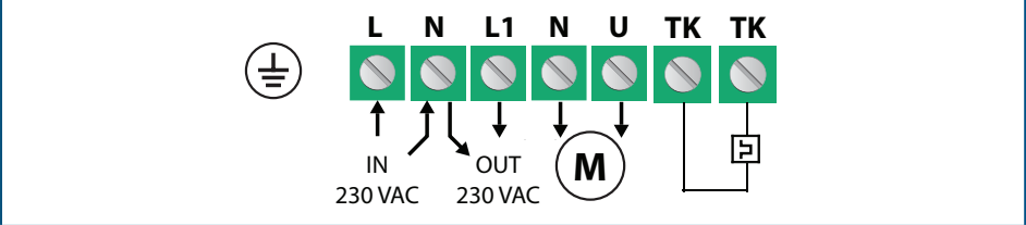
Fig. 3 Wiring and connections
