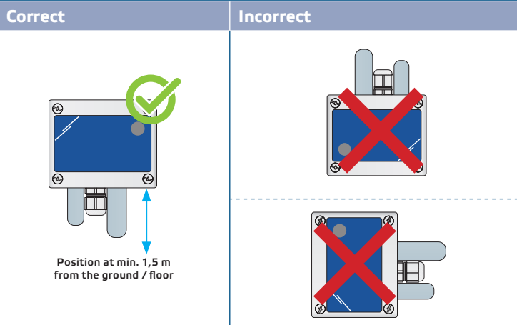
Fig. 2 Mounting position
