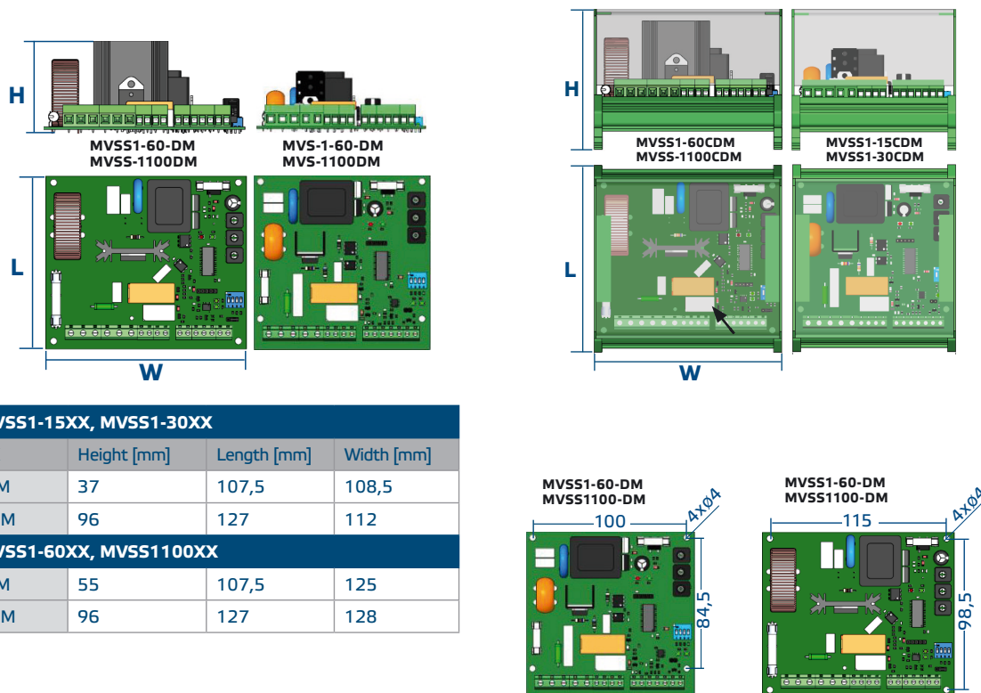
Fig. 1 Mounting dimensions
