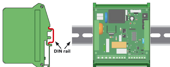
Fig. 2 Mounting position
