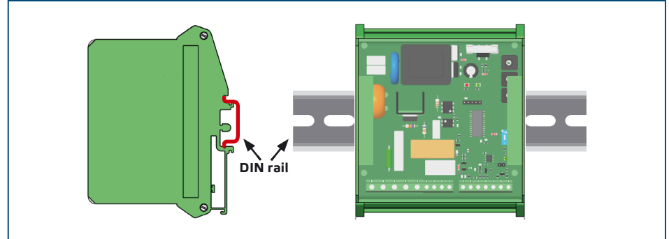
Fig. 2 Mounting position
