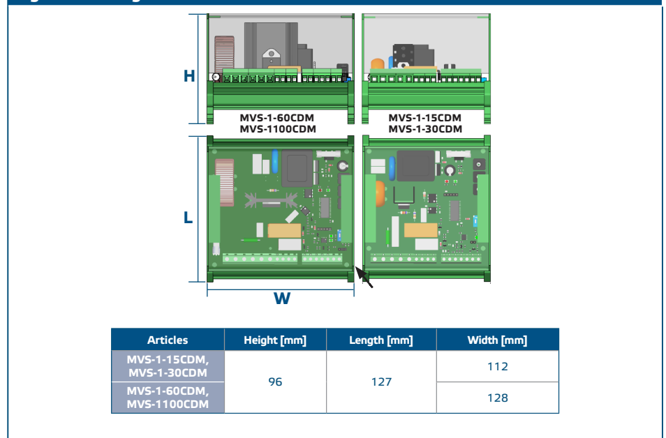
Fig. 1 Mounting dimensions
