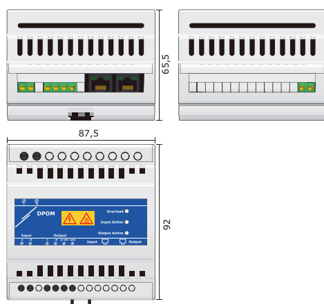
Fig. 1 Mounting dimensions
