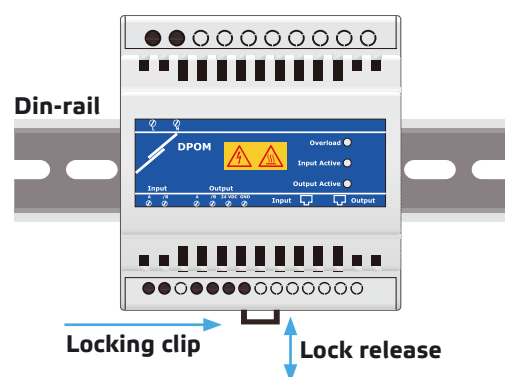
Fig. 2 Mounting position
