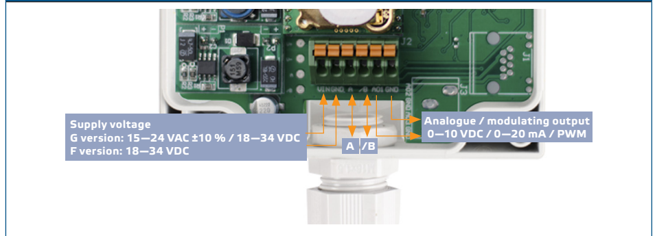
Fig. 4 Wiring and connections
