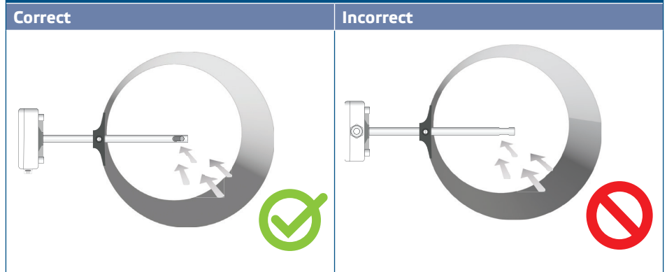
Fig. 2 Mounting position
