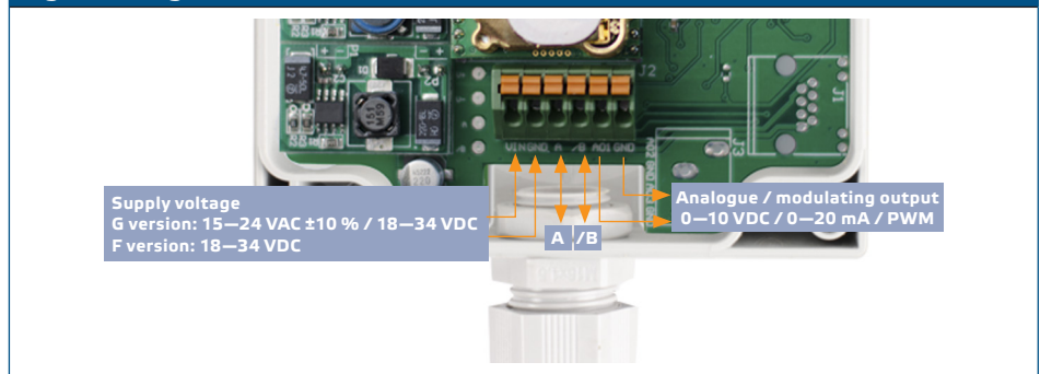
Fig. 4 Wiring and connections
