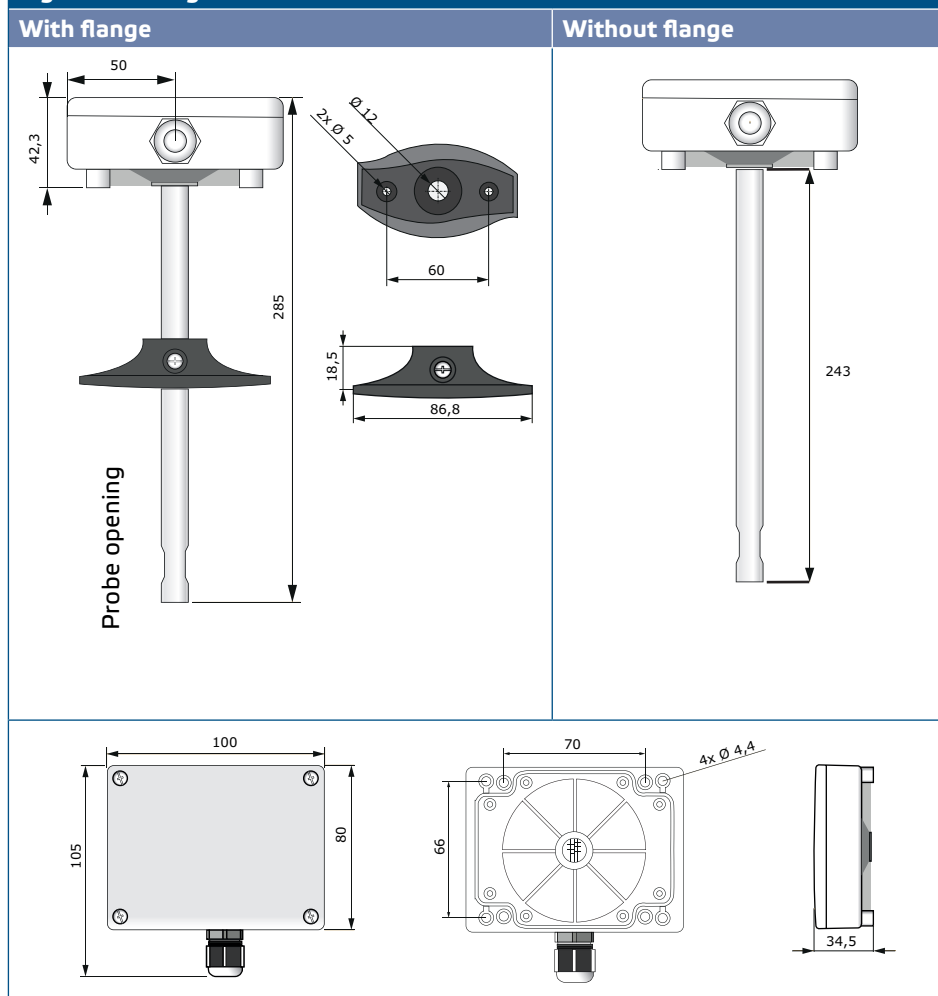
Fig. 1 Mounting dimensions
