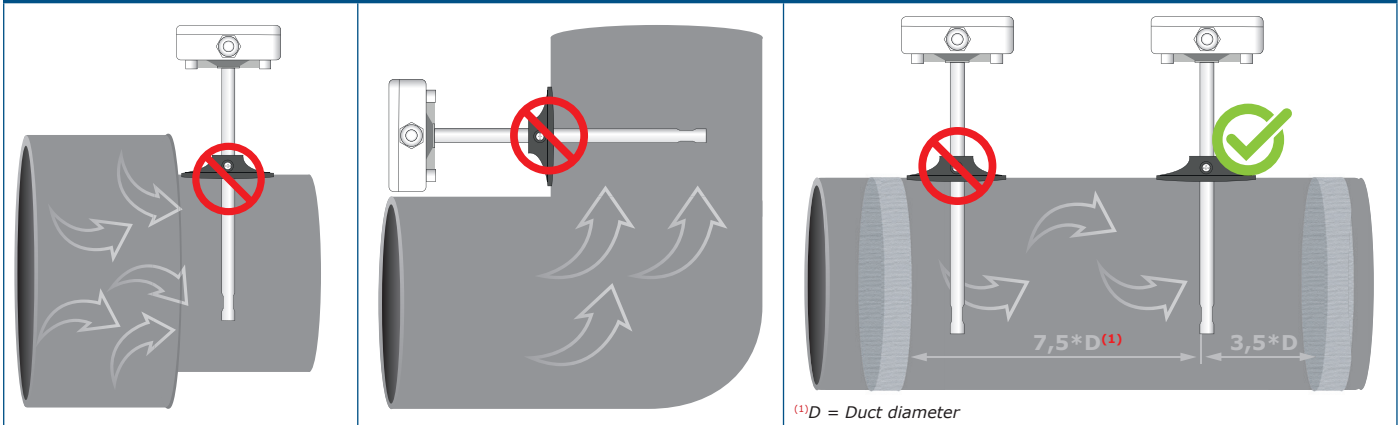
Fig. 3 Mounting requirements
