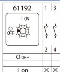
Switching diagram 61192
