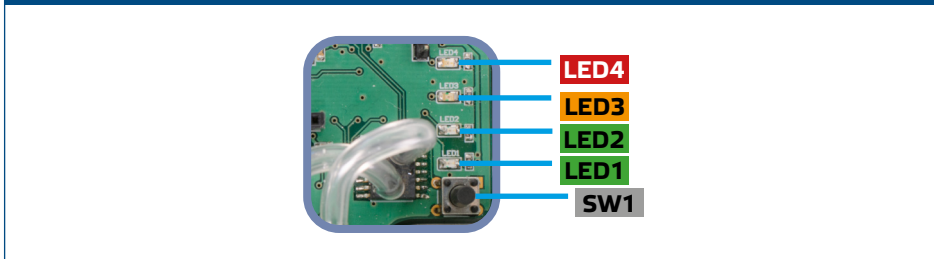
Obr. 9 LED indikace
